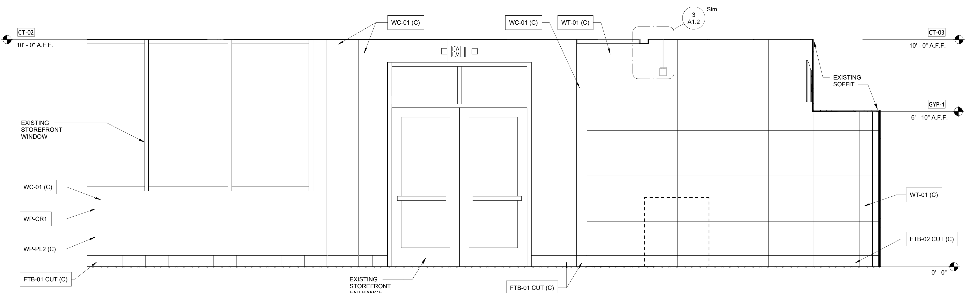
2 A4.1 1/2" = 1'-0"
