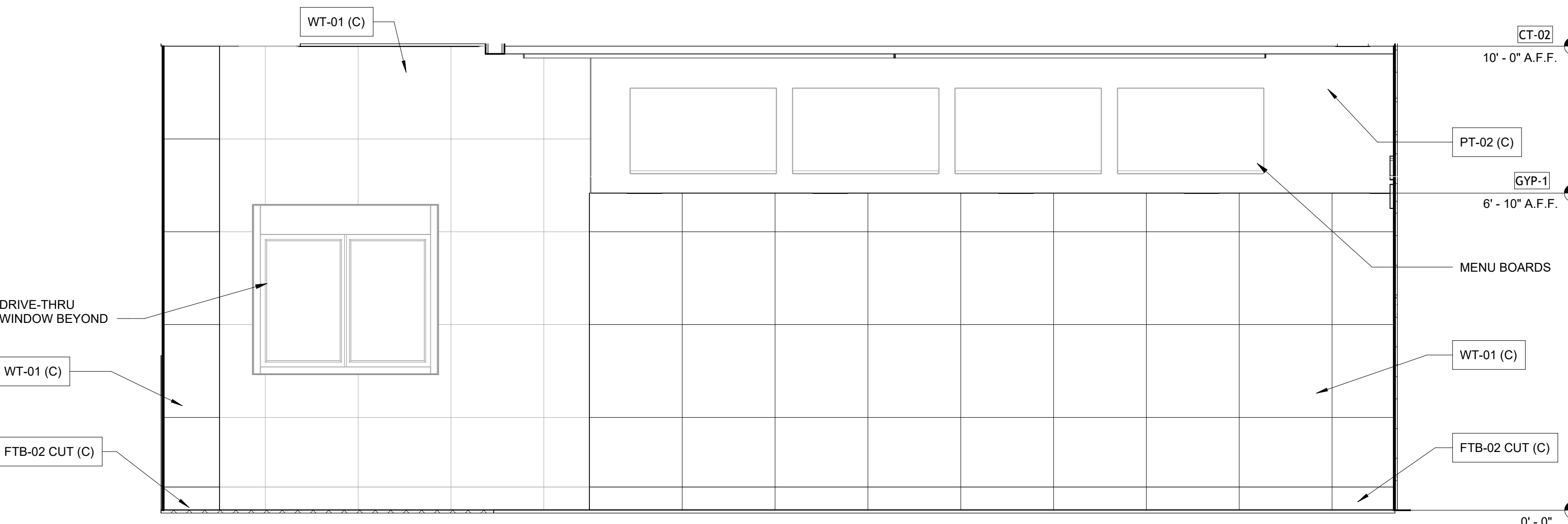
1 A4.1 1/2" = 1'-0"
