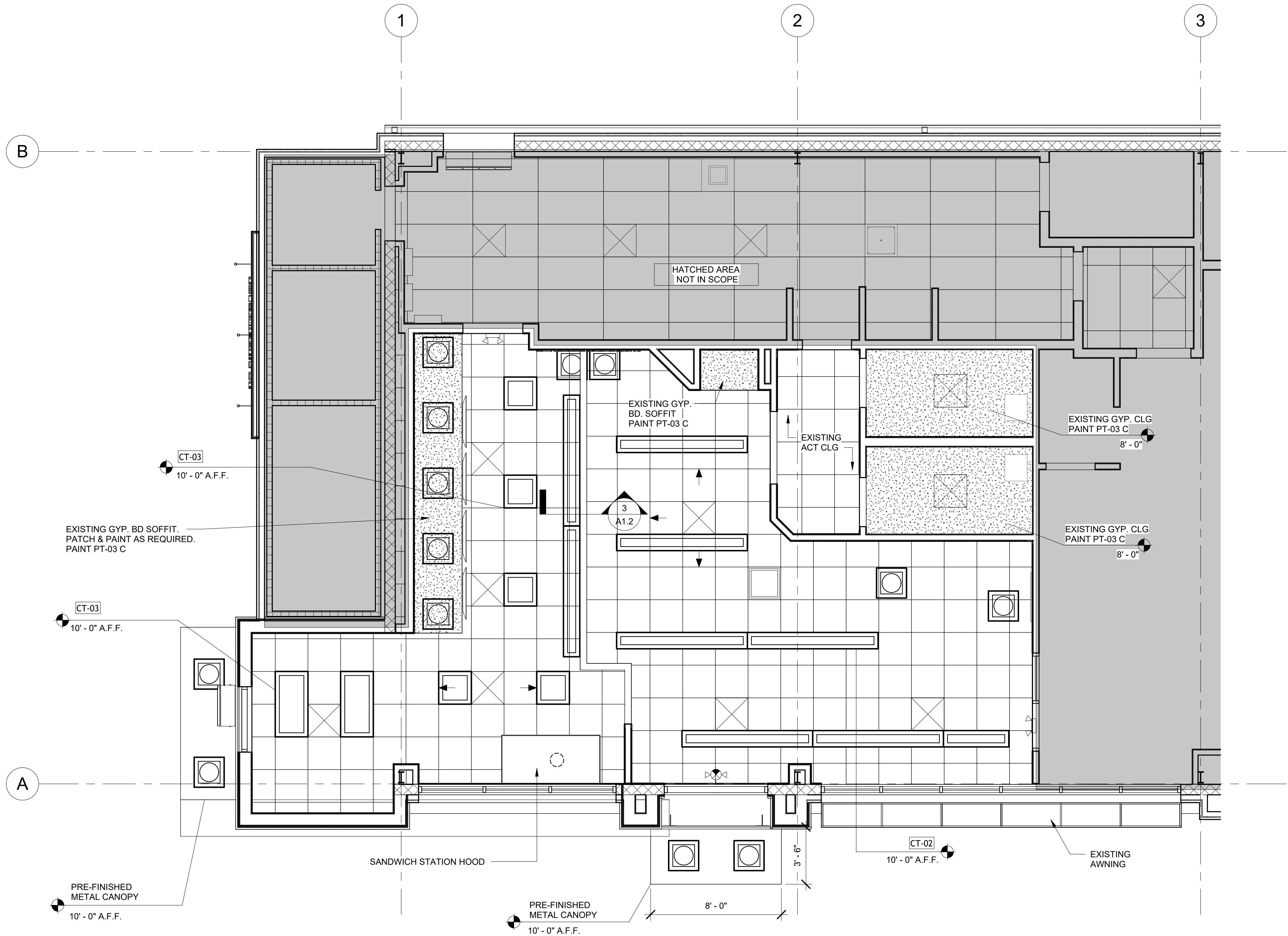
1 A1.2 1/4" = 1'-0" REFLECTED CEILING PLAN
