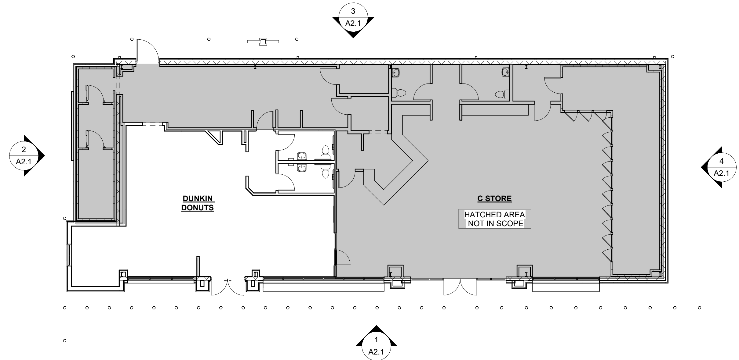
2 A1.1 OVERALL FLOOR PLAN 3/32" = 1'-0"
