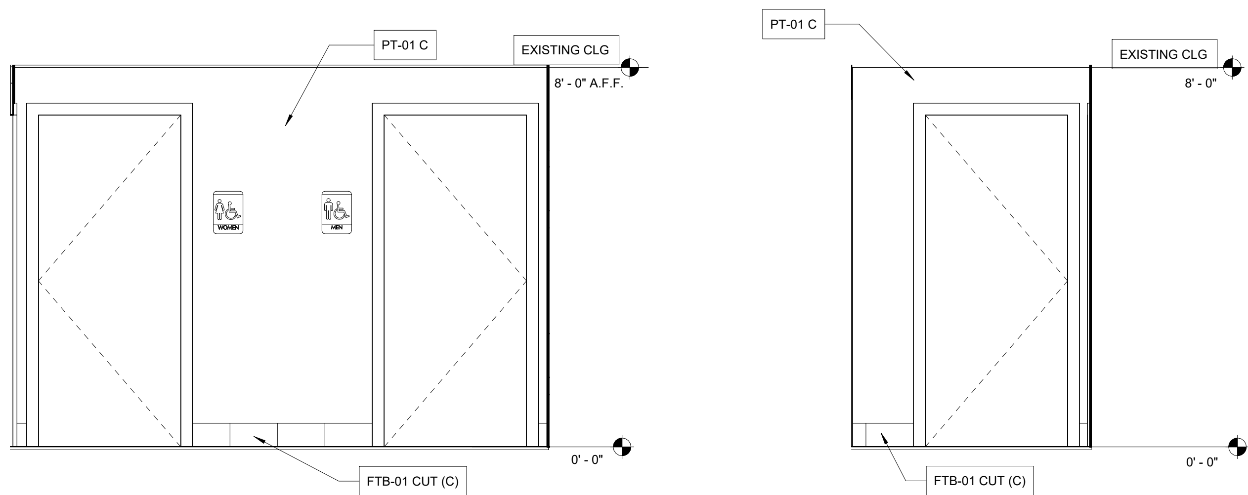
6 A4.1 1/2" = 1'-0"
