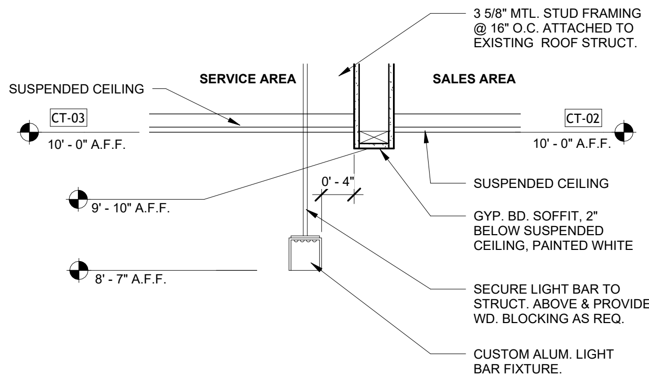
3 A1.2 1" = 1'-0" INTERIOR SOFFIT DETAIL
