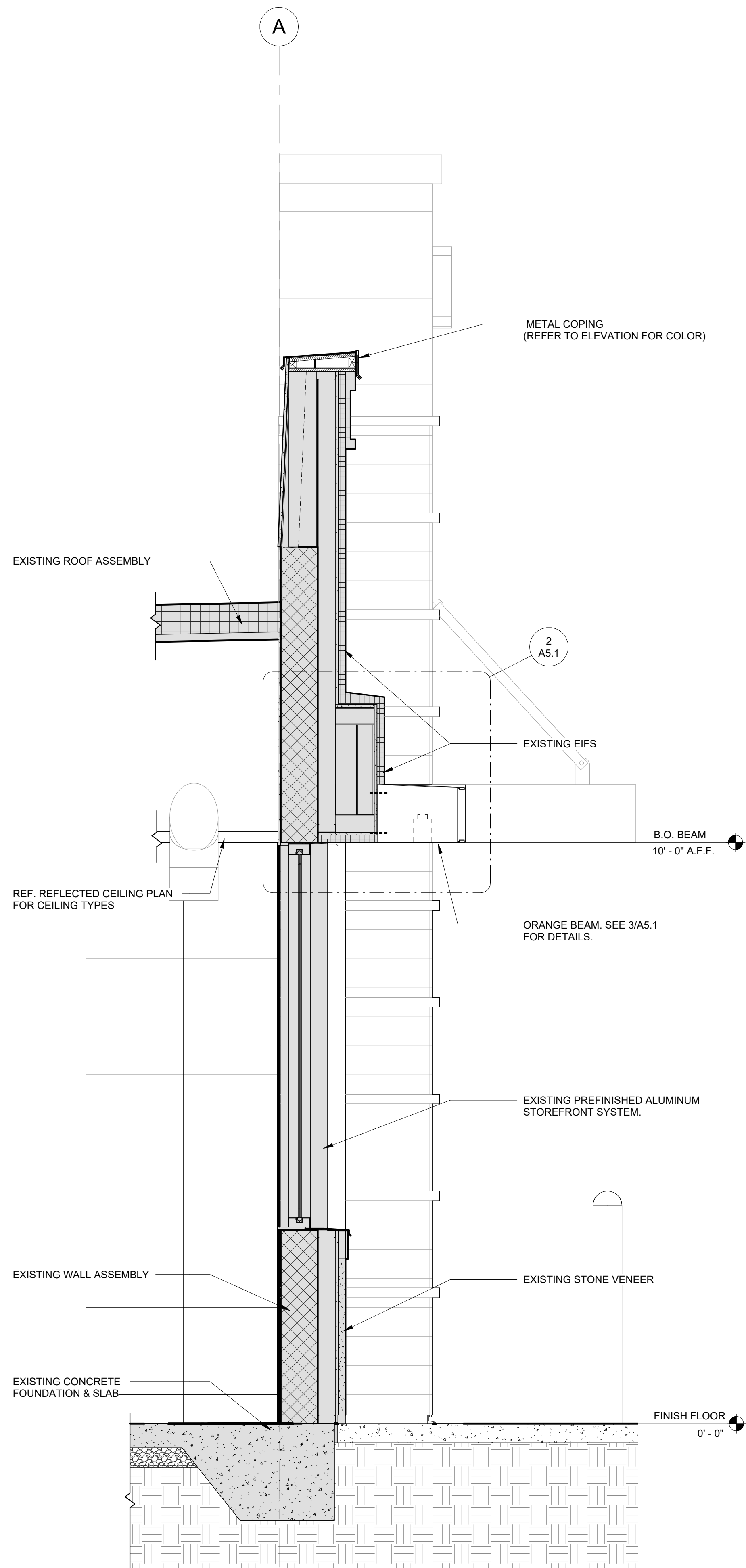
2 WALL SECTION 3/4" = 1'-0"
