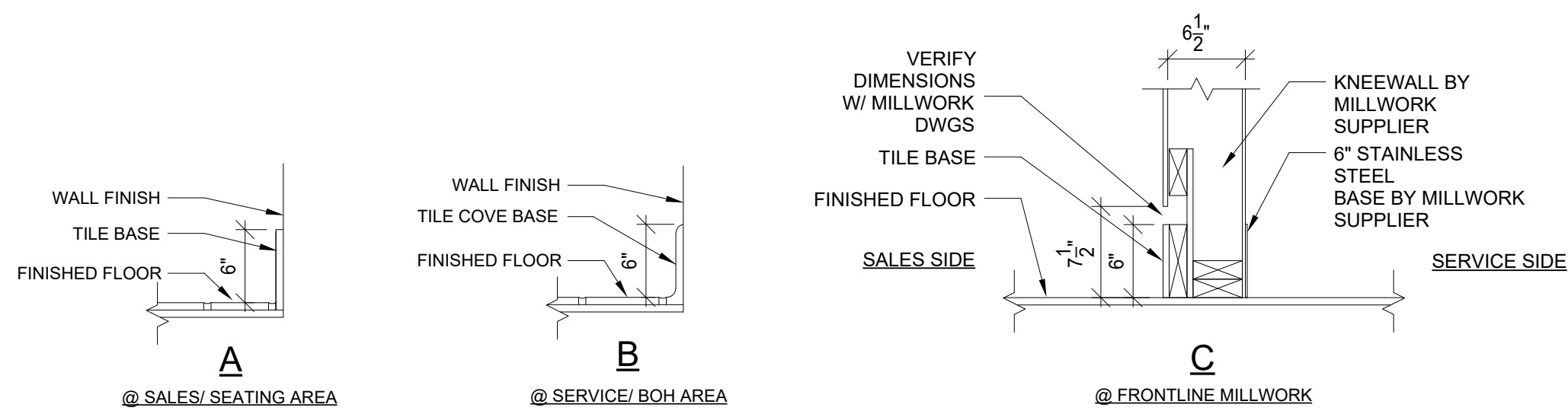
TILE BASE DETAIL
