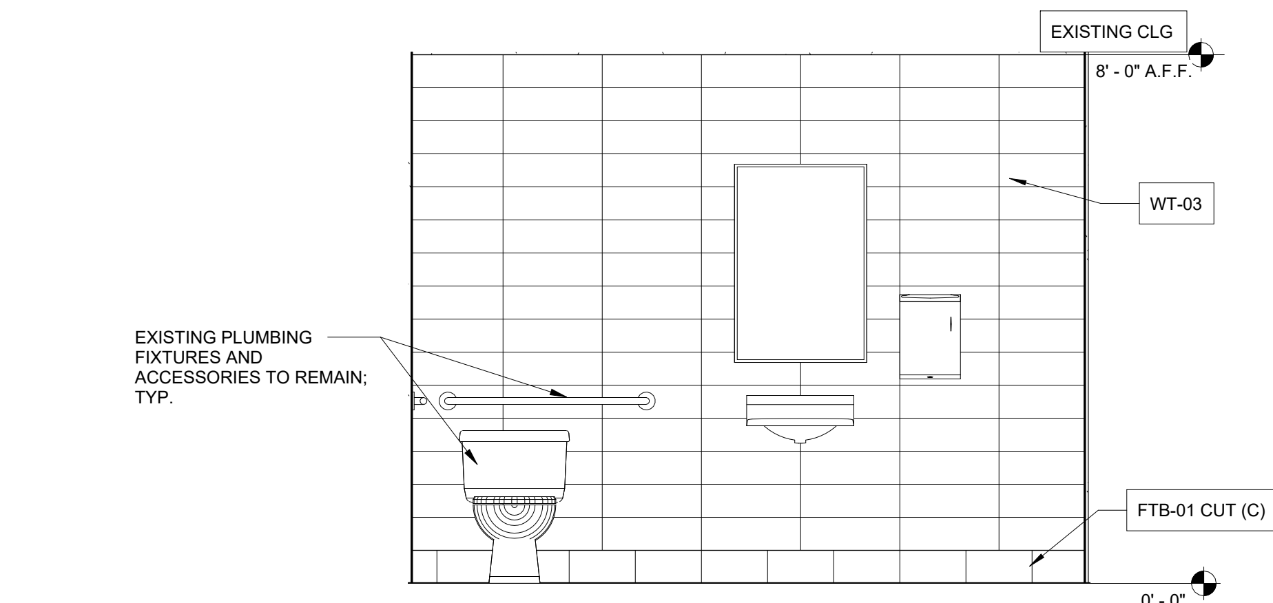
8 A4.1 1/2" = 1'-0"
