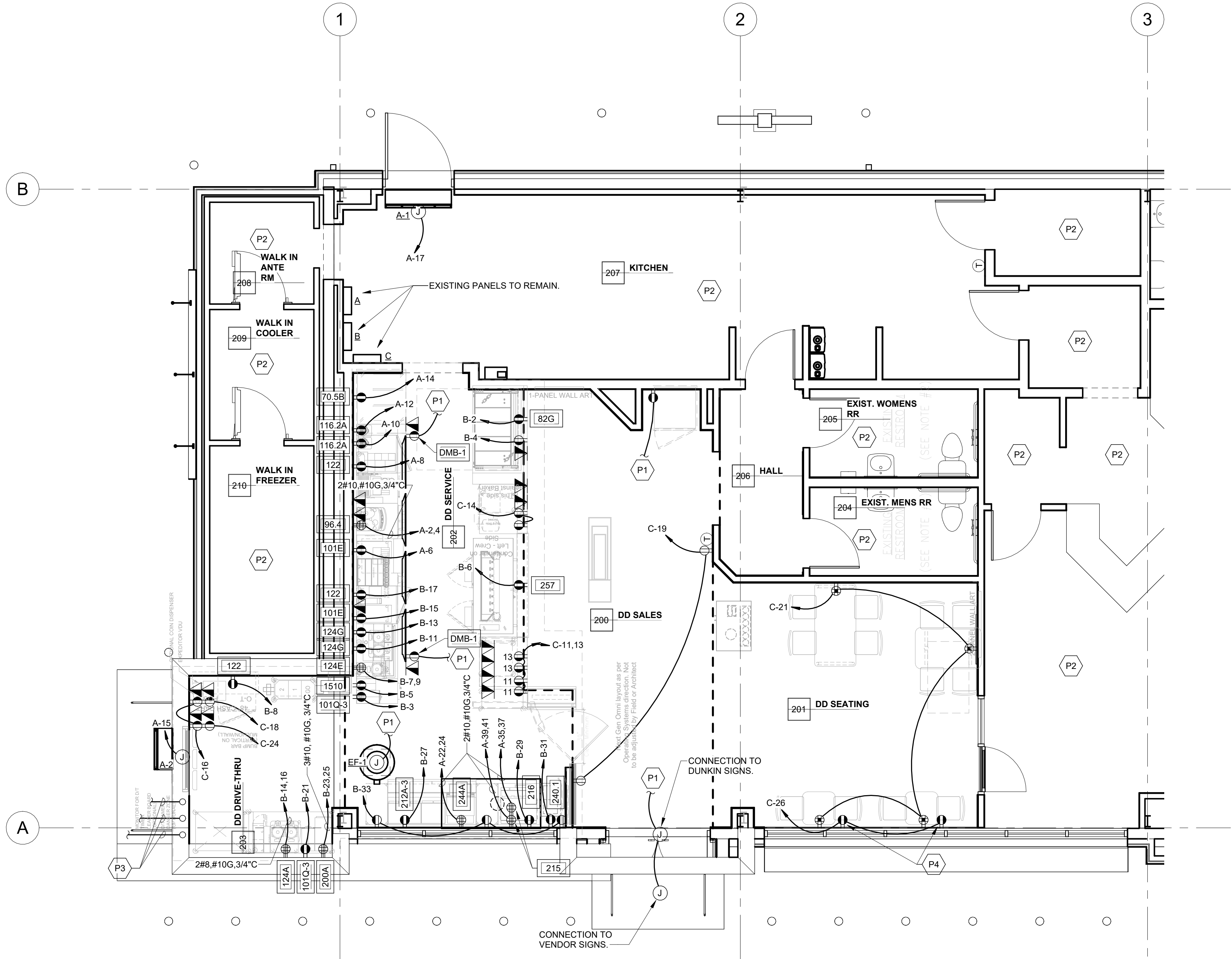
1 POWER PLAN E2.1 1/4" = 1'-0"
