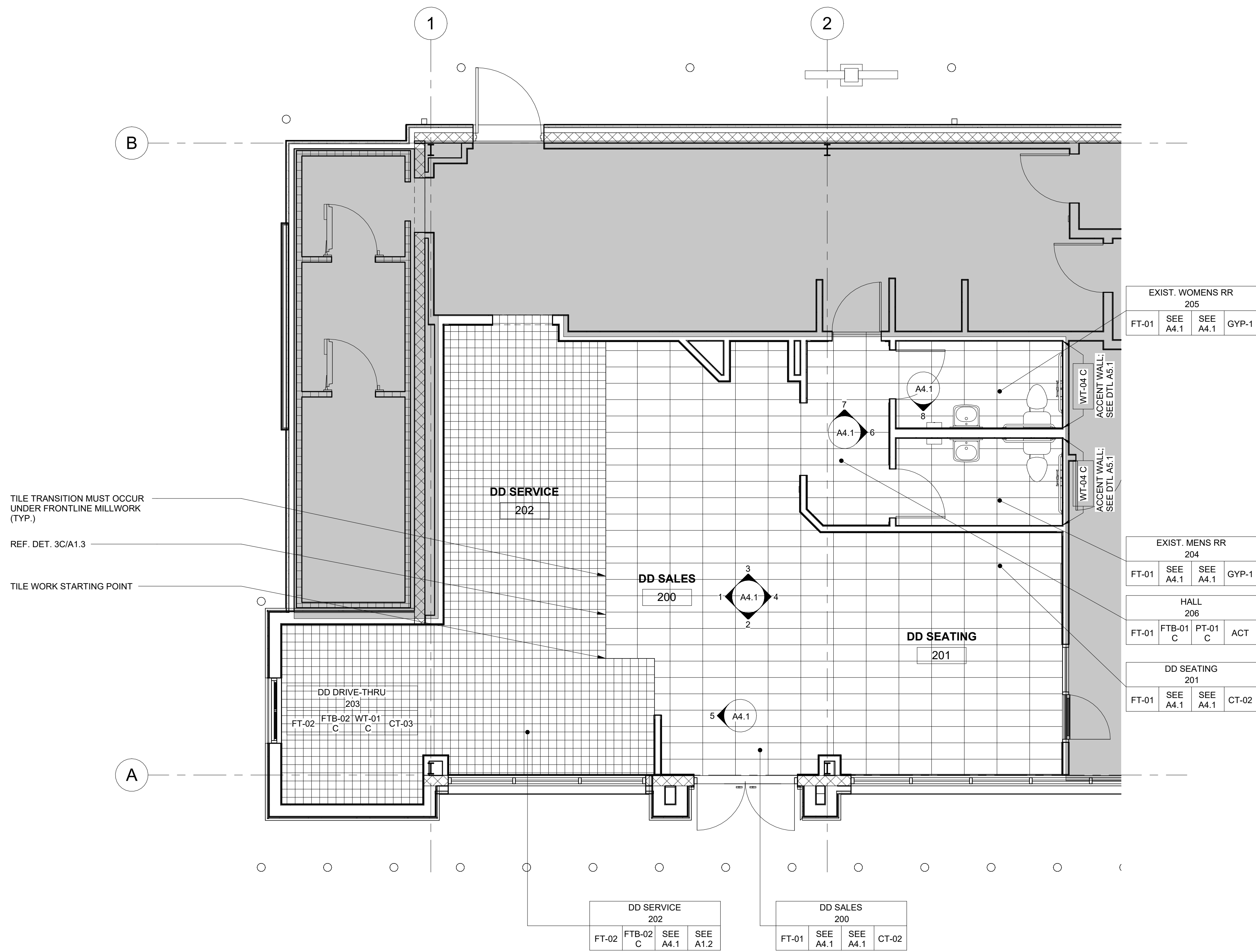
FLOOR PLAN FINISH 1/4" = 1'-0"
