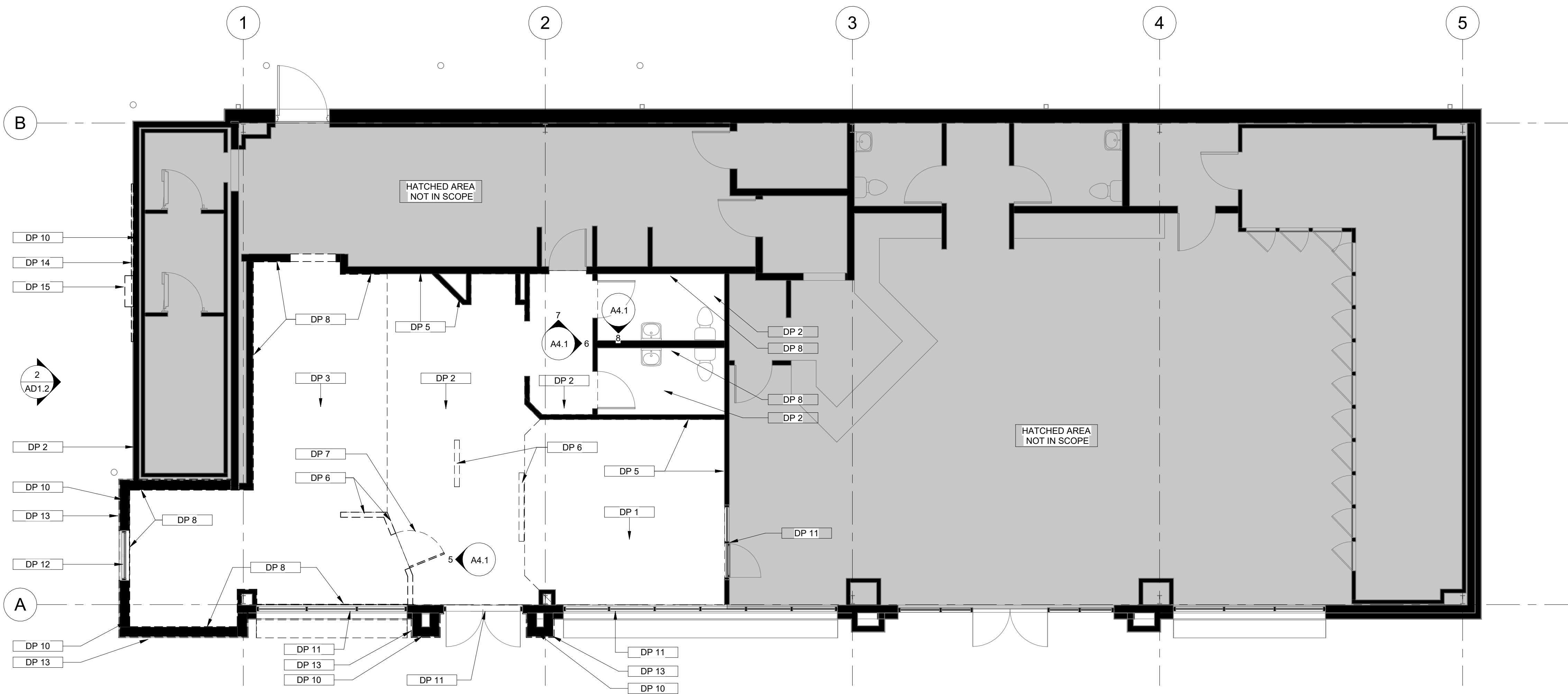
FLOOR PLAN DEMO
