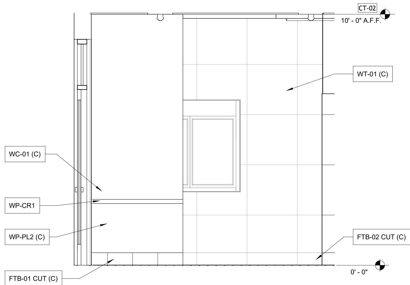
5 A4.1 1/2" = 1'-0"
