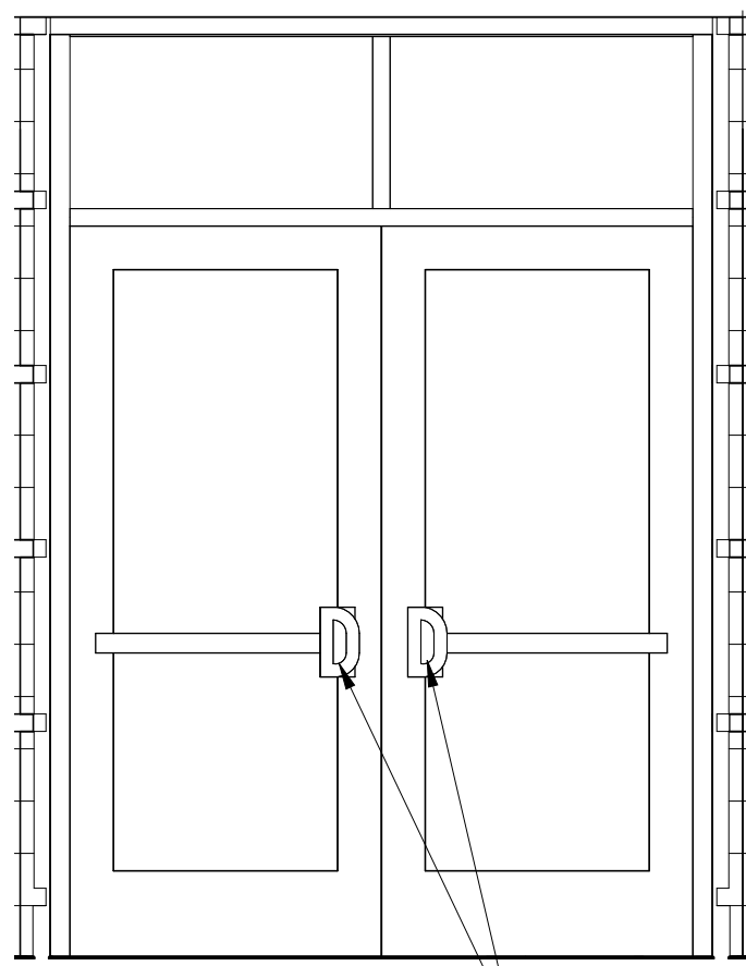
4 A1.1 DOOR HANDLE DETAIL 1/2" = 1'-0"
