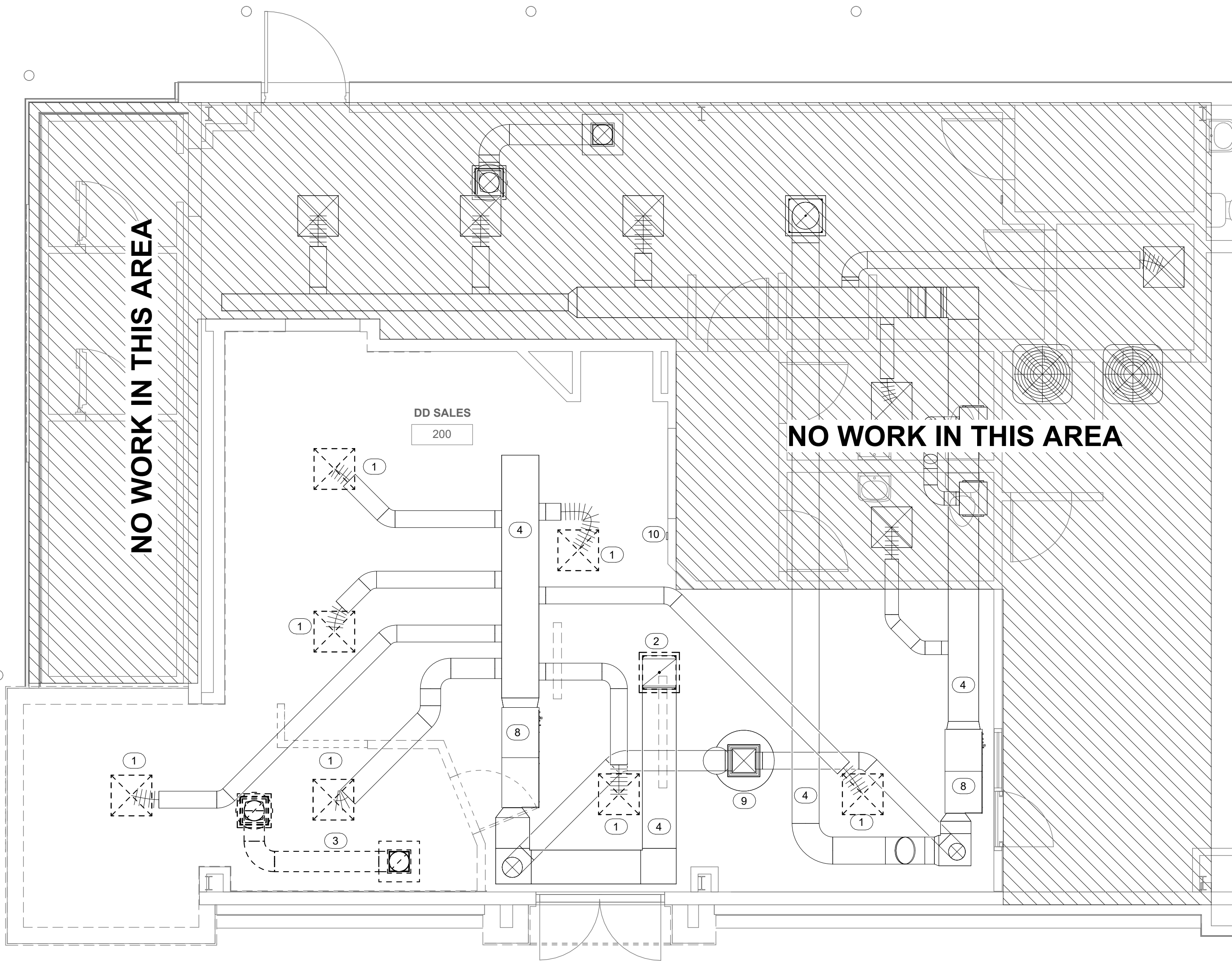
1 HVAC - DEMOLITION FLOOR PLAN 1/4" = 1'-0"
