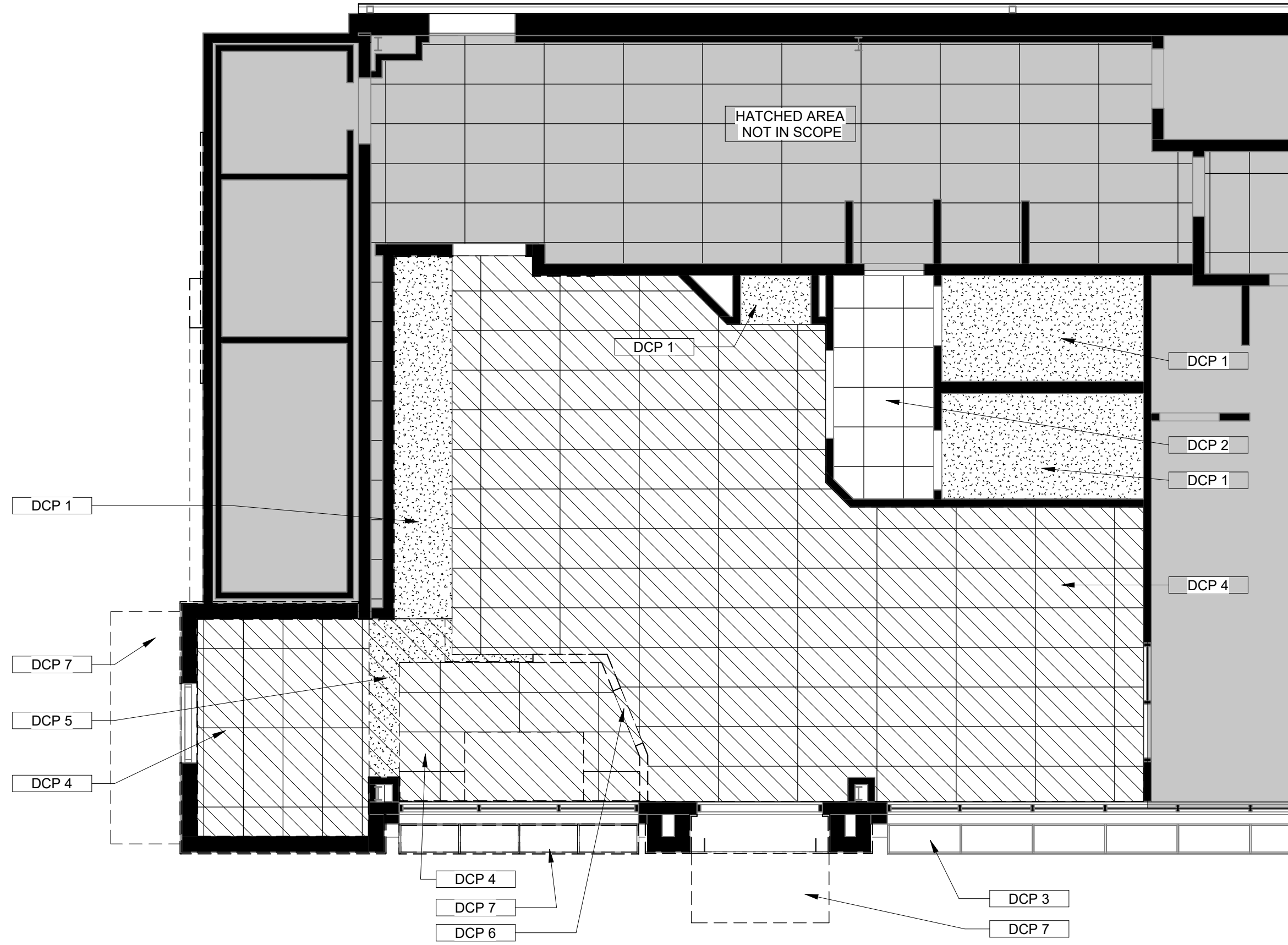
2 REF CLG PLAN DEMO AD1.1 3/16" = 1'-0"
