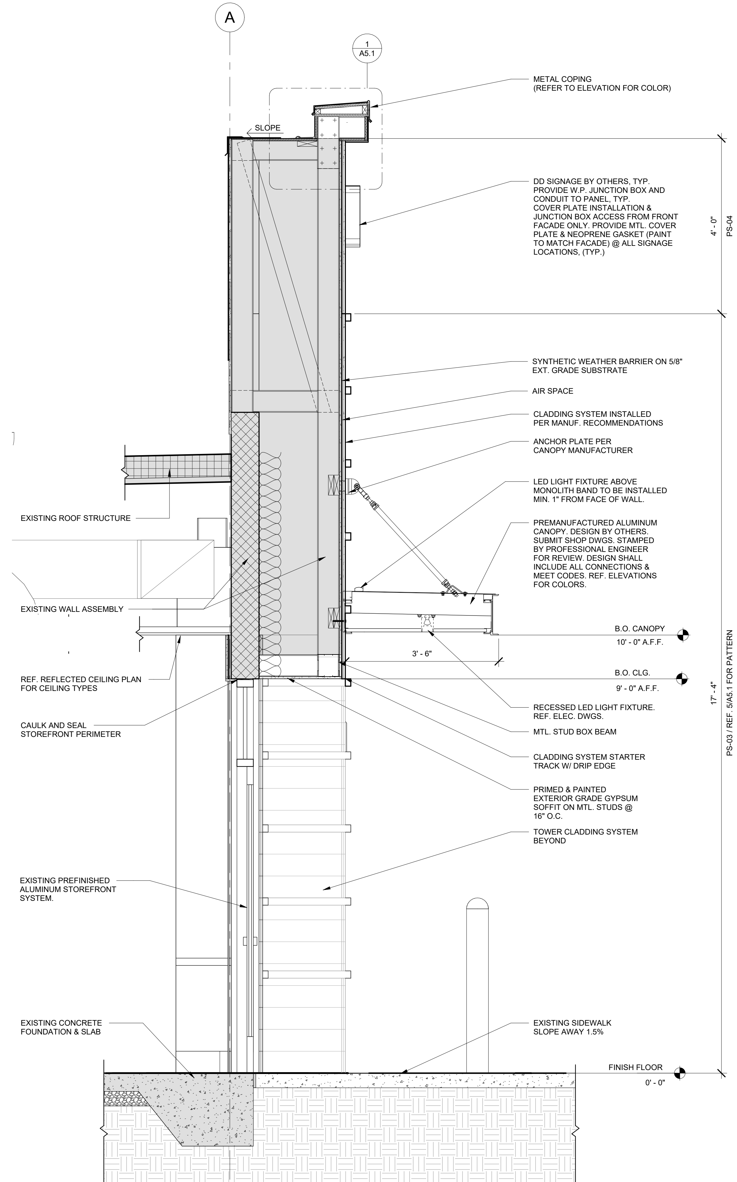
1 WALL SECTION 3/4" = 1'-0"
