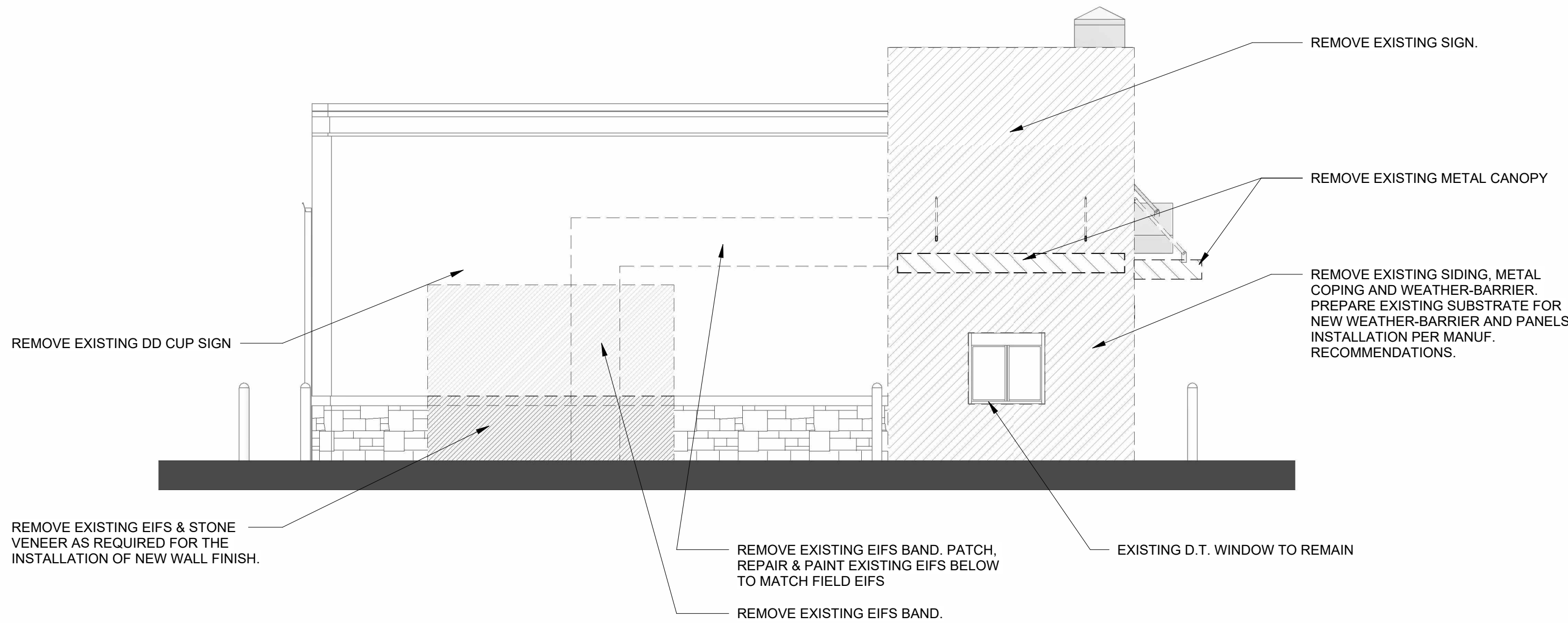
2 SIDE ELEVATION - DEMO AD1.2 3/16" = 1'-0"
